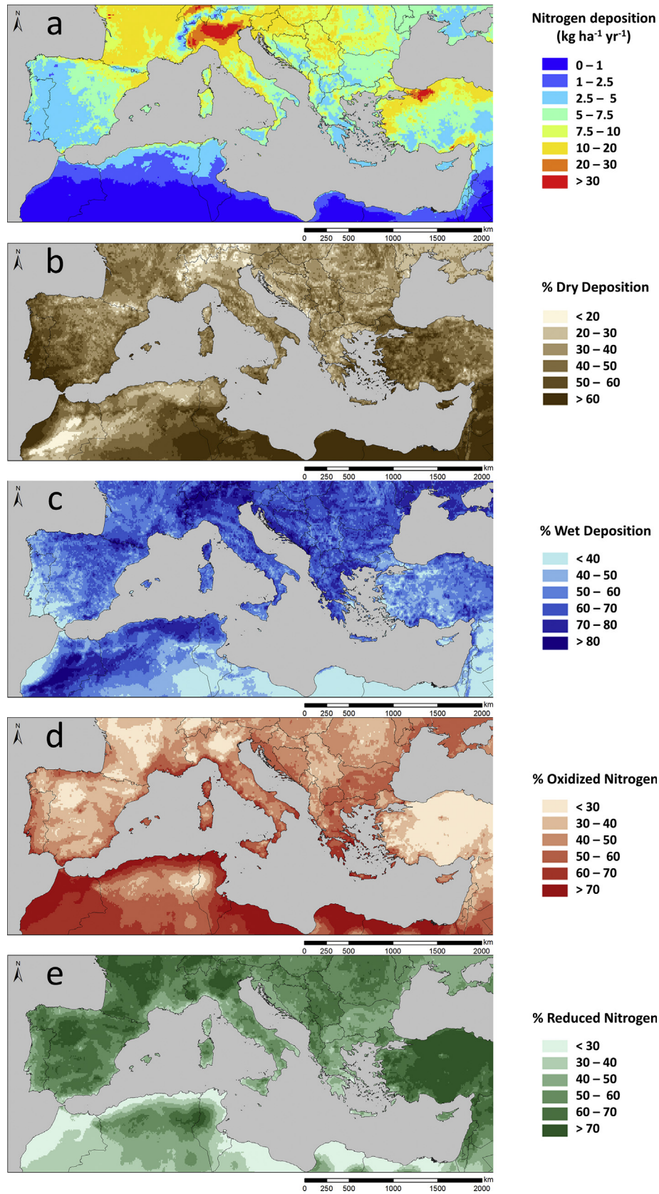
Fig. 1. Modelled nitrogen deposition for the Mediterranean region based on the European Monitoring and Evaluation Programme (EMEP) model at 0.1°-0.1° longitude-latitude resolution (EMEP MSC-W chemical transport model [version rv4.7; www.emep.int ]). Modelled N deposition is based on 2013 emissions data. (a) Total N deposition (oxidized + reduced; dry + wet), (b) percentage of dry deposition, (c) percentage of wet deposition, (d) percentage of oxidized deposition and (e) percentage of reduced deposition.
