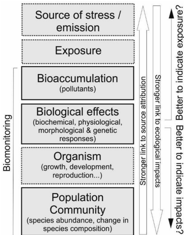
Fig. 4. The biomonitoring chain: from the source of stress to ecological impacts. Measurements closer to the source of stress (e.g. bioaccumulation of pollutants) have a stronger link to source attribution, provide an account of exposure, and can be seen as an early warning system for potential impacts. On the other hand, biological effects (biomarkers) and species-based measurements commonly have a close link to impacts on the ecosystem but can have a weaker link to source attribution. Dark frame indicates those levels and measurements most commonly considered in biomonitoring studies.
